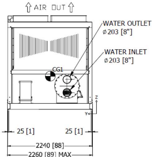
LEFT VIEW
