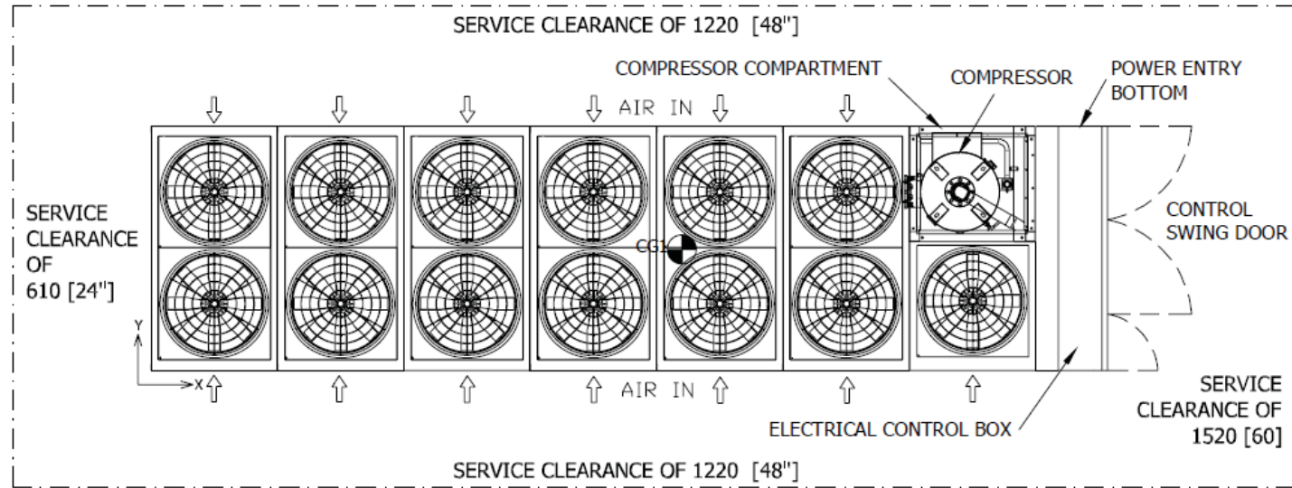
TOP VIEW
